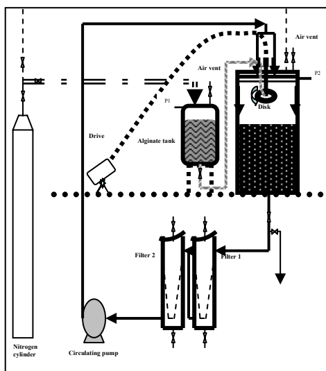
Fig. 5. The UWS Prototype Encapsulator.
